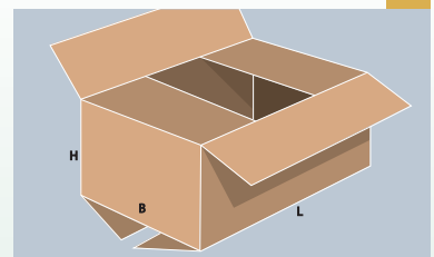
Folding carton FEFCO 0201 with abutting base and cover flaps
